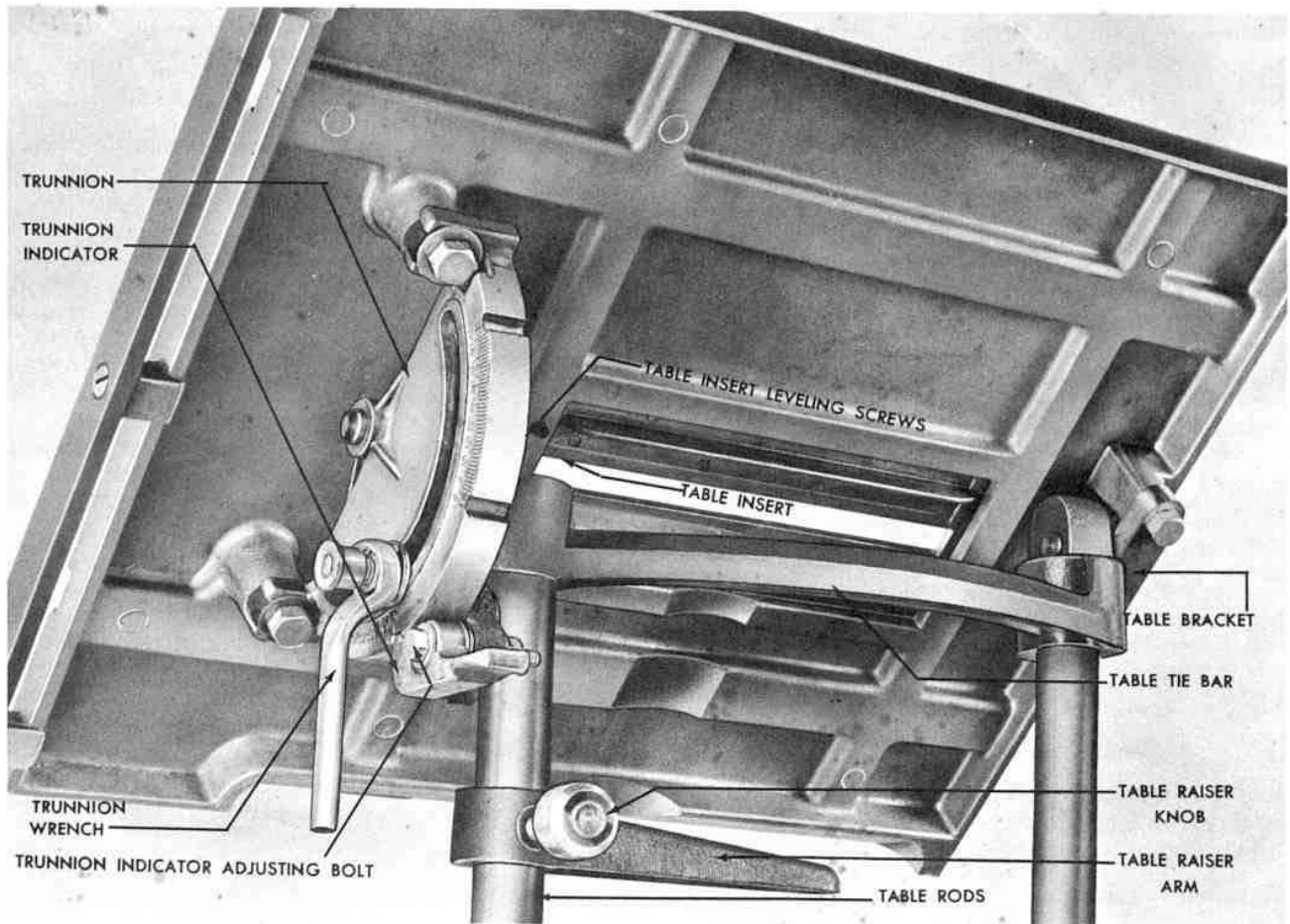
Underside of saw table (tilted) with parts designated.
